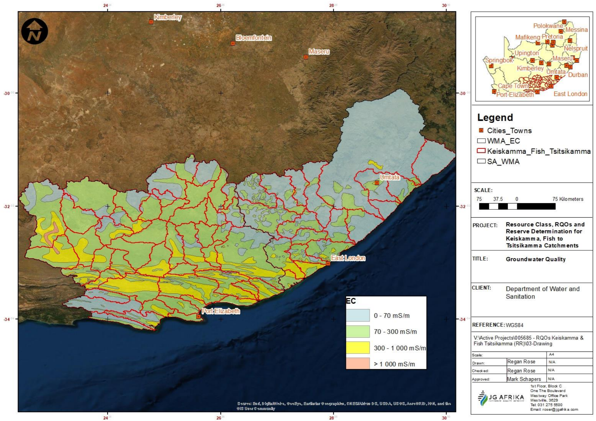
Figure 11-8: Groundwater quality
